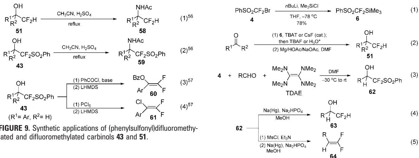
FIGURE 10. Nucleophilic (phenylsulfonyl)difluoromethylation with reagents 4 and 6 .
